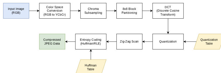
JPEG Scheme
